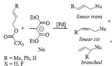
Scheme 3. Pd-catalysed allylic alkylation with sodium diethyl 2-methylmalonate as the nucleophile
