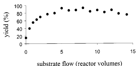
Figure 5. Application of dendrimeric ligand 20 in the allylic amination of crotyl acetate and piperidine in a continuous-flow membrane reactor ( P/Pd = 4 , yield in % conversion of crotyl acetate in the product stream)
