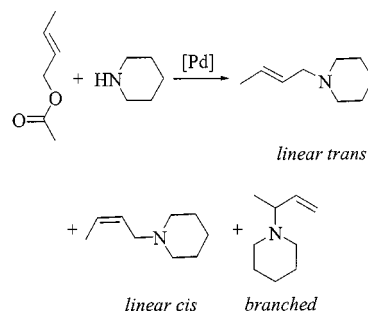
Scheme 4. Pd-catalysed allylic amination with piperidine as the nucleophile
