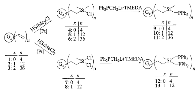
Scheme 1. Synthesis of diphenylphosphane-functionalised carbosilane dendrimers with a methylene spacer between Si atom and P atom
