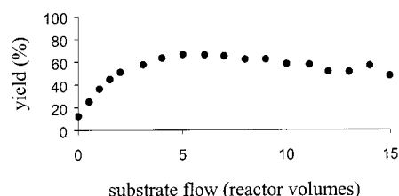
Figure 4. Application of dendrimeric ligand 20 in the allylic amination of crotyl acetate and piperidine in a continuous-flow membrane reactor ( \text{P/Pd} = 2 , yield in % conversion of crotyl acetate in the product stream)
