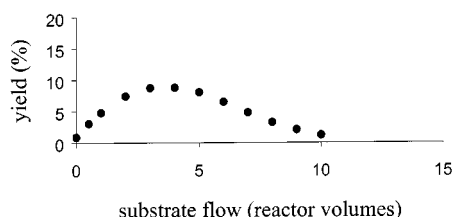
Figure 3. Application of dendrimeric ligand 13 in the allylic amination of crotyl acetate and piperidine in a continuous-flow membrane reactor (yield in % conversion of crotyl acetate in the product stream)
