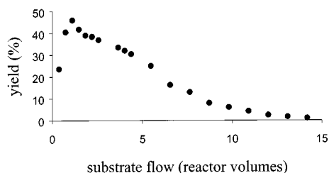
Figure 2. Application of dendrimeric ligand 13 in the allylic alkylation of allyl trifluoroacetate and sodium diethyl 2-methylmalonate in a continuous-flow membrane reactor (yield in % conversion of allyl trifluoroacetate in the product stream)
