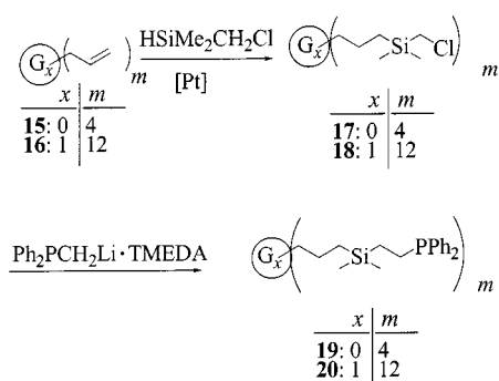
Scheme 2. Synthesis of diphenylphosphane-functionalised carbosilane dendrimers with an ethylene spacer between the Si atom and the P atom
