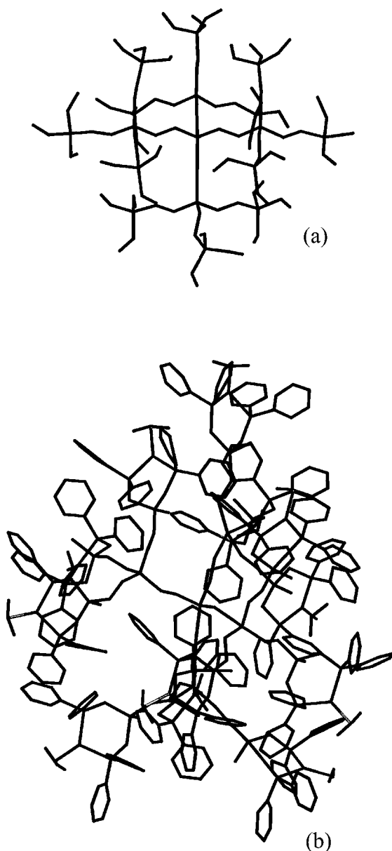
Figure 1. Crystal structure of the second generation dendrimer 3 (a) and a modelled structure [58] of the (allyl)Pd complex of 13 (b); hydrogen atoms and counter ions have been omitted for clarity
